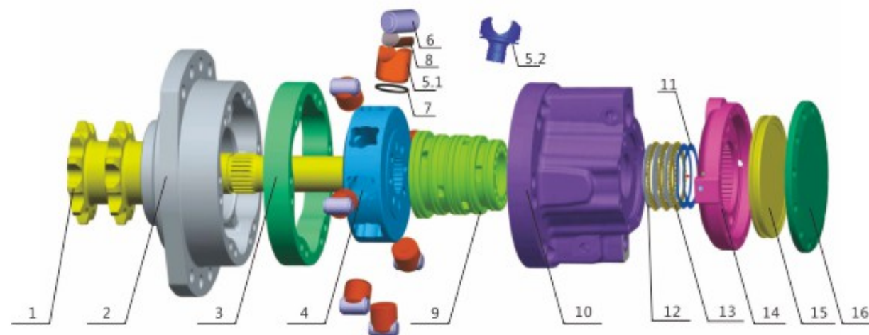
HMCRO5/HMCRE05 系列零件名称表 HMCRO5/HMCRE05 series parts list
