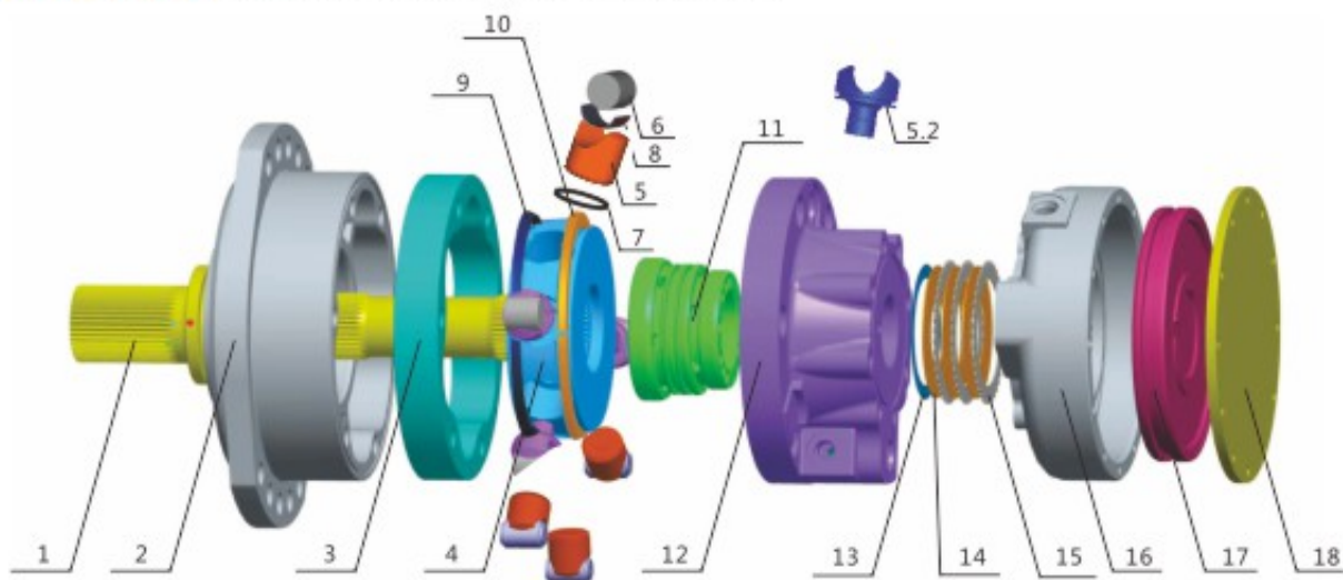
HMCRO3/HMCRE03 系列零件名称表 HMCRO3/HMCRE03 series parts list
