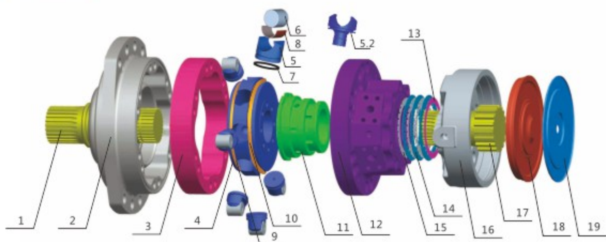
HMCR10/HMCRE10 系列零件名称表 HMCR10/HMCRE10 series parts list
